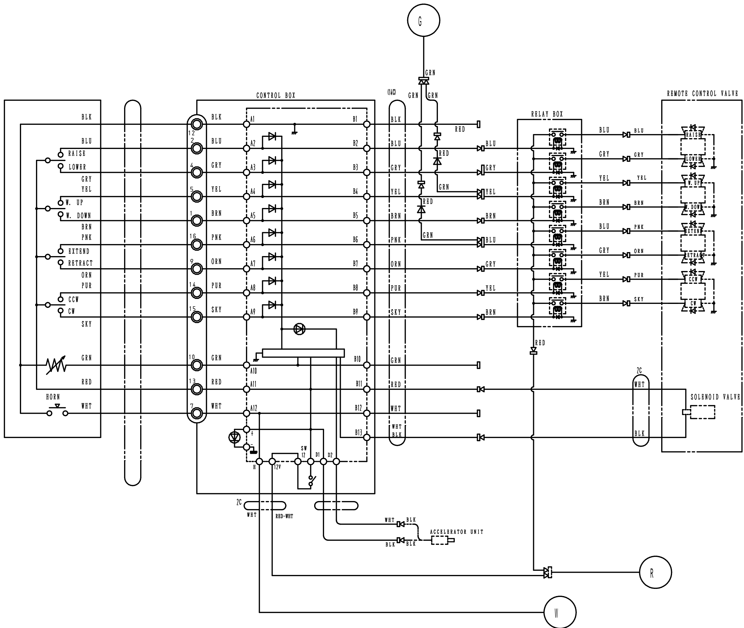
ELECTRIC DIAGRAM (REMOTE CONTROL SYSTEM)
