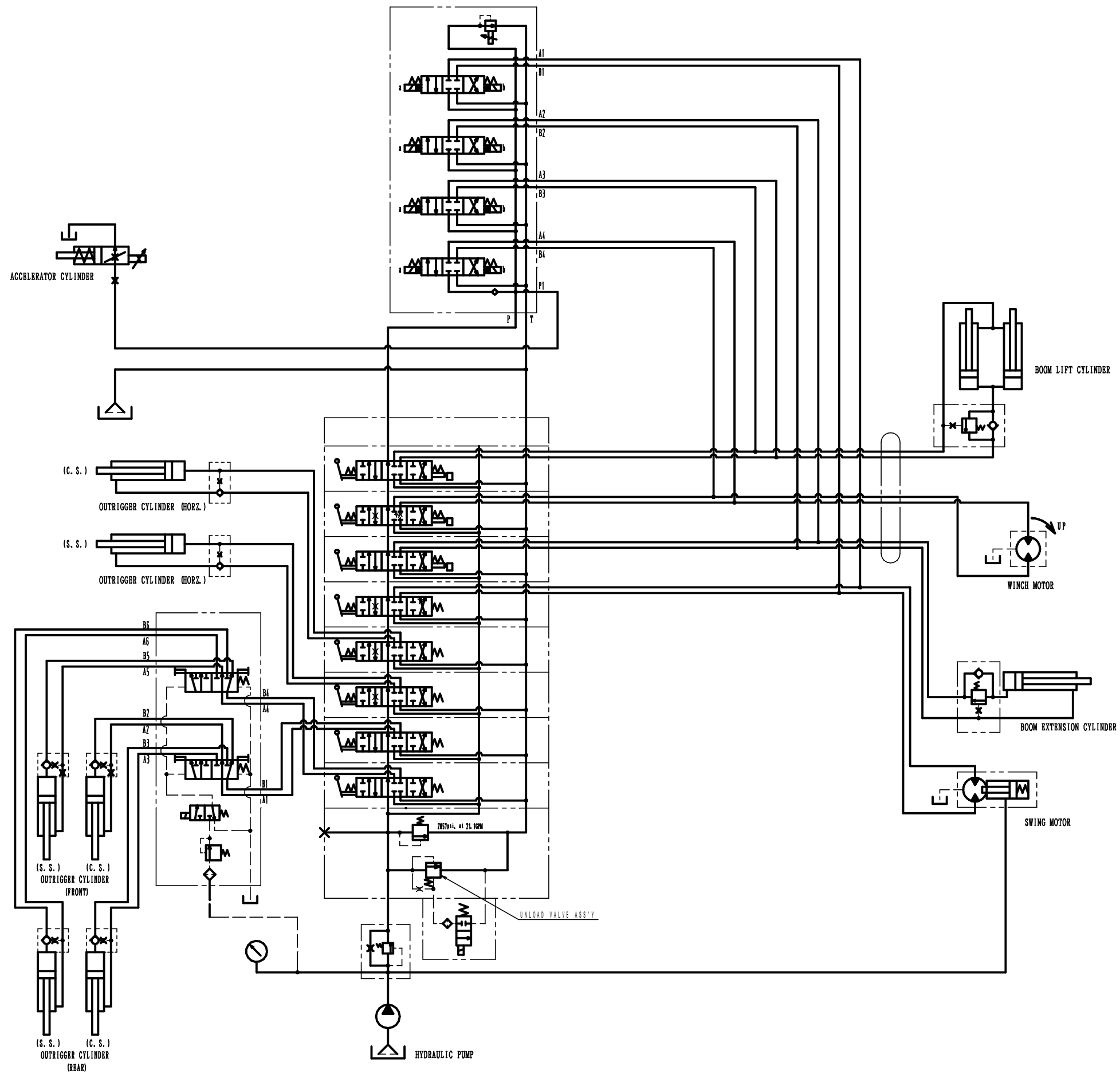
UR800R HYDRAULIC DIAGRAM
