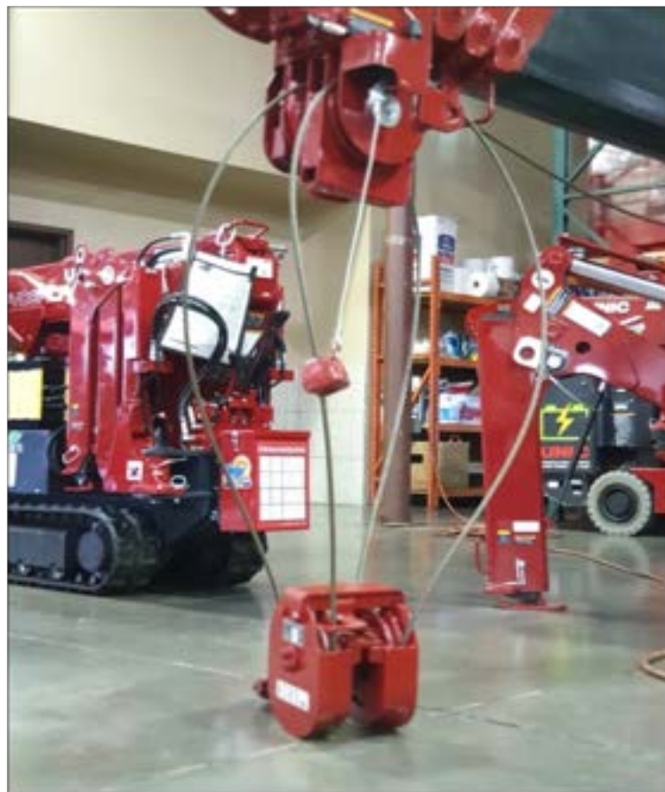
(Fig. 2): BOOM DOWN to actually place the hook block on the ground.
