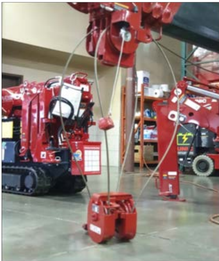
(Fig. 1): NEVER lift the hook block off the ground via WINCHING UP; ALWAYS BOOM UP/BOOM OUT to un-ground the hook block.
