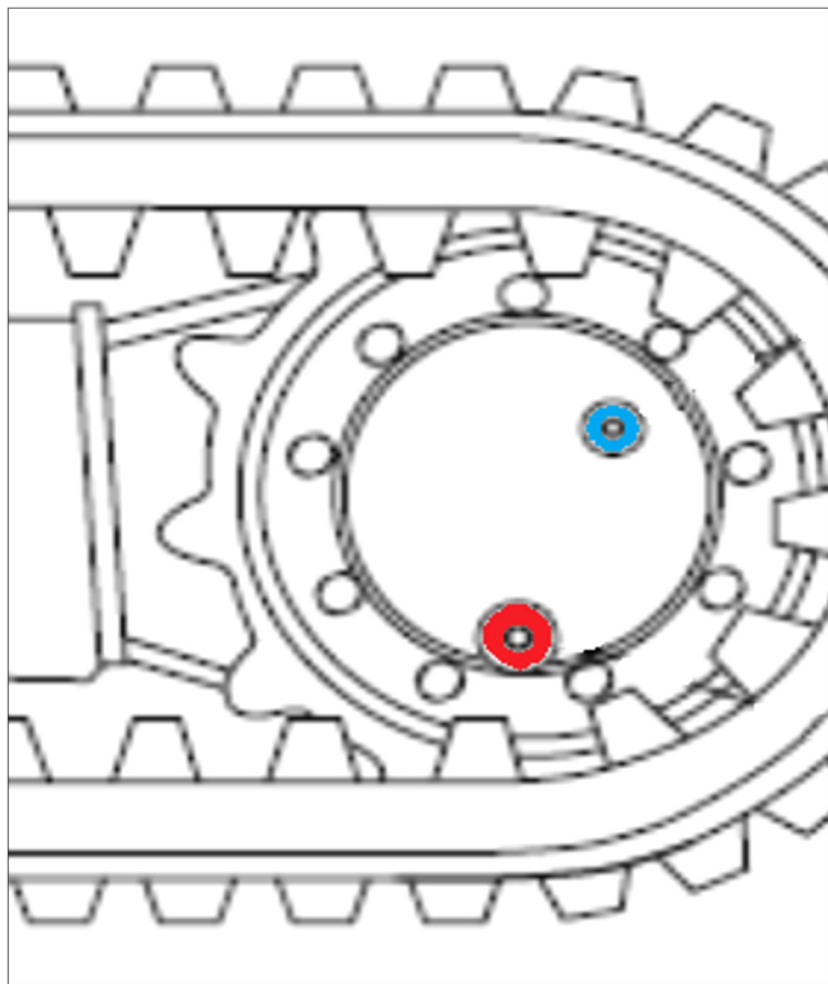
(Fig. 1): The larger Drain Port should be at the 6 o'clock position before it's plug is removed.
