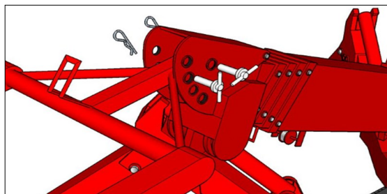
(Fig. 2): Place and orient the AWP so that it is directly in front of the SPYDERCRANE with the end of the yoke pointing at the Boom Tip.
