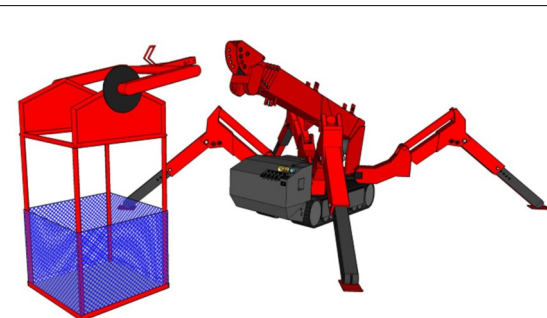
(Fig. 1): Place and orient the AWP so that it is directly in front of the SPYDERCRANE with the end of the yoke pointing at the Boom Tip.
