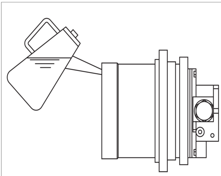
(Fig. 2): After replacing the Drain Port Plug, add oil through the Fill Port until the Drive Wheel is filled.
